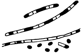
FIG. 112.—SPORES OF BACILLUS ANTHRACIS , \times 1200 ; stained with gentian-violet, after passing the cover-glass twelve times through the flame.
